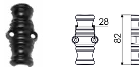
J0545.. Coulant RY59
