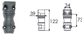
J055191 Chapiteau RY220
